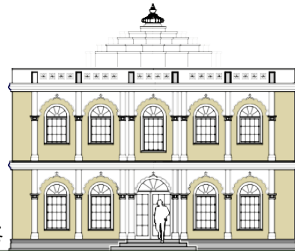
East Elevation
