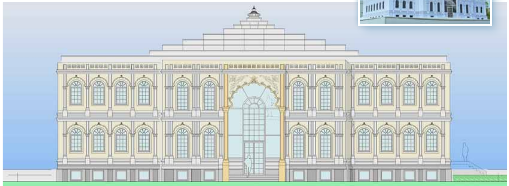
East Elevation – Length 33m /Depth 18m
